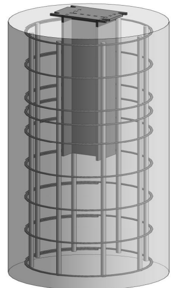
FDOT Multi Column Foundation
