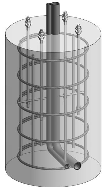
FDOT Pedestrian Foundation
