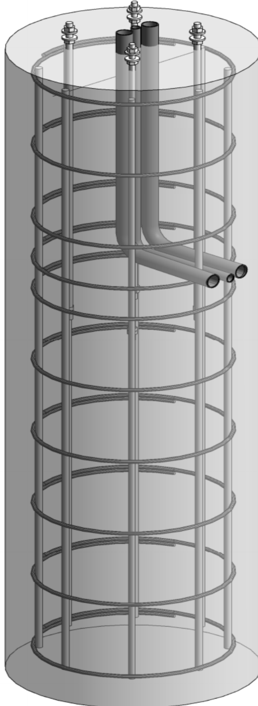
FDOT and Commercial Light pole Foundations
